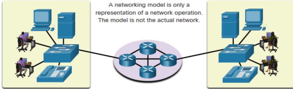
OSI Model
