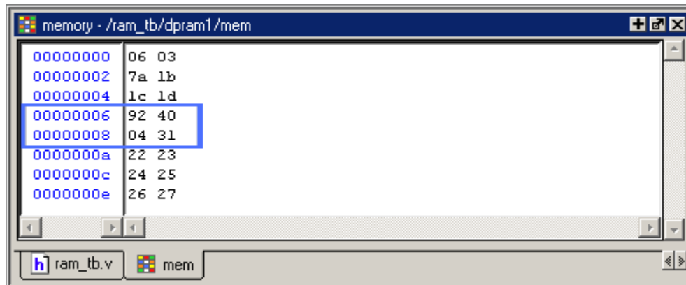
Figure 7-15. Random Content Generated for a Range of Addresses
