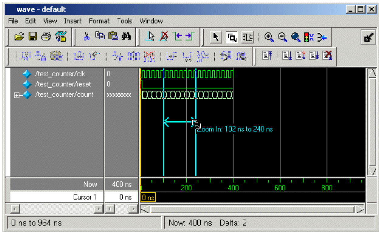
Figure 6-3. Zooming in with the Mouse Pointer
