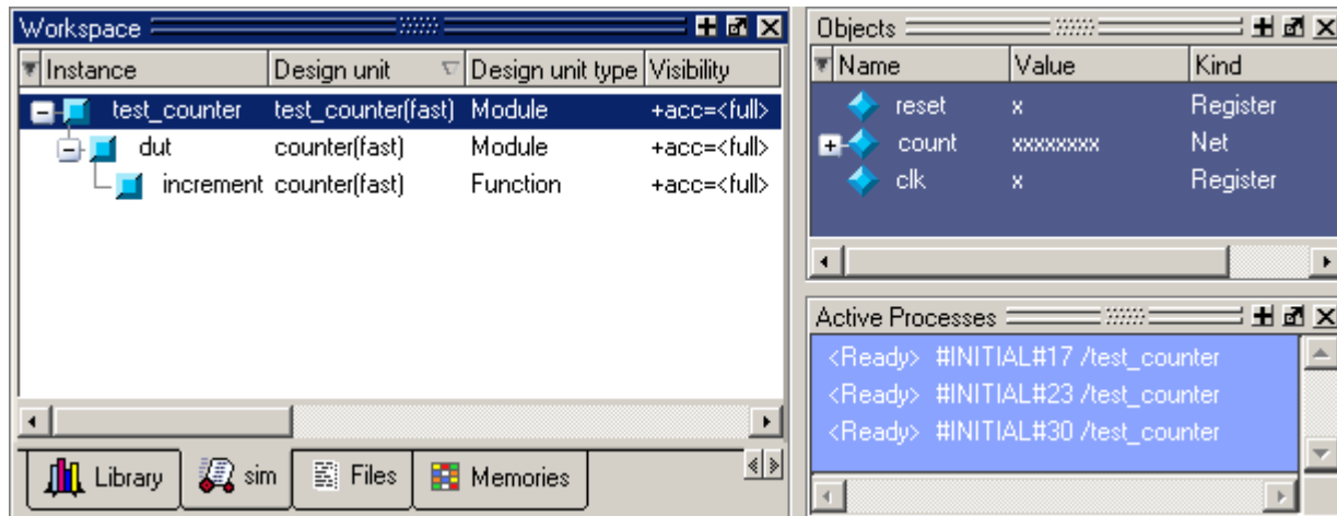
Figure 3-7. Workspace and Objects Panes Showing a Verilog Design
