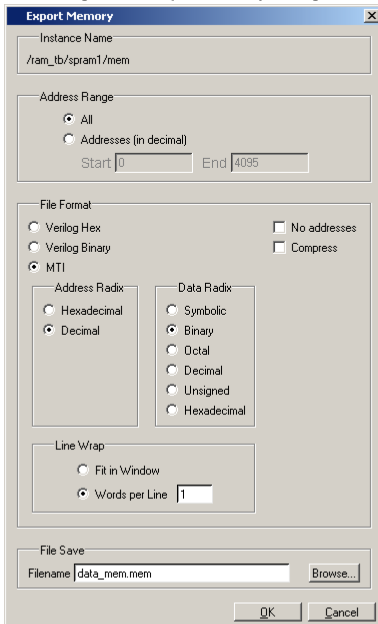
Figure 7-9. Export Memory Dialog
