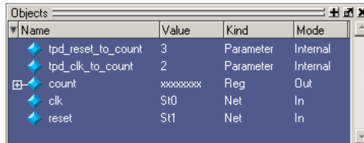
Figure 3-13. Values Shown in Objects Window
