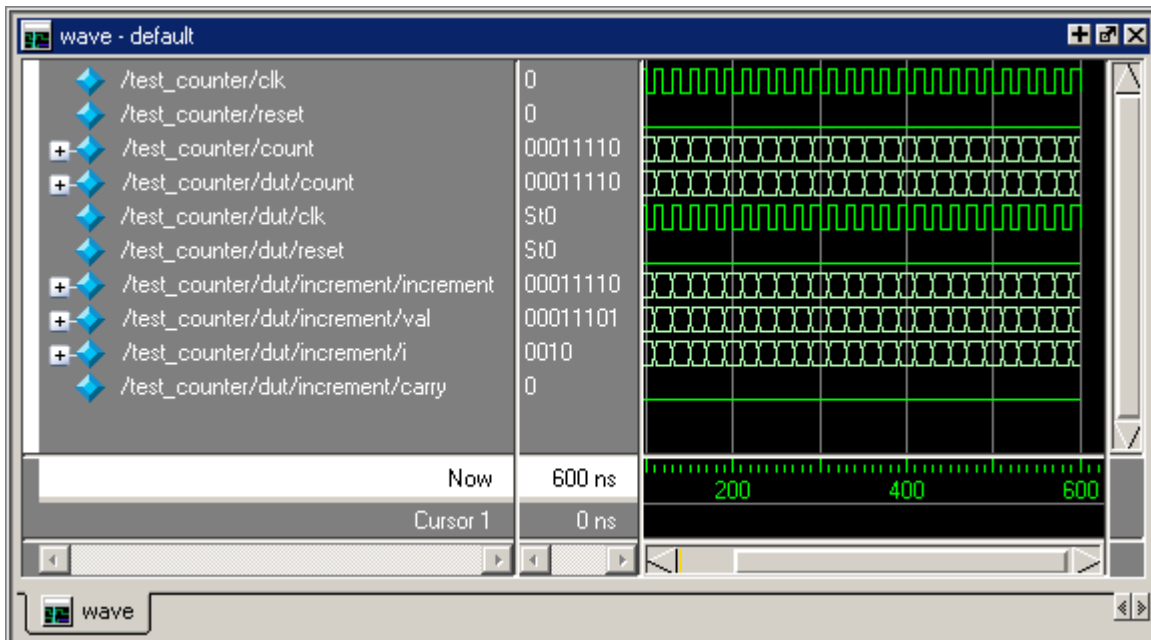
Figure 3-9. Waves Drawn in Wave Window
